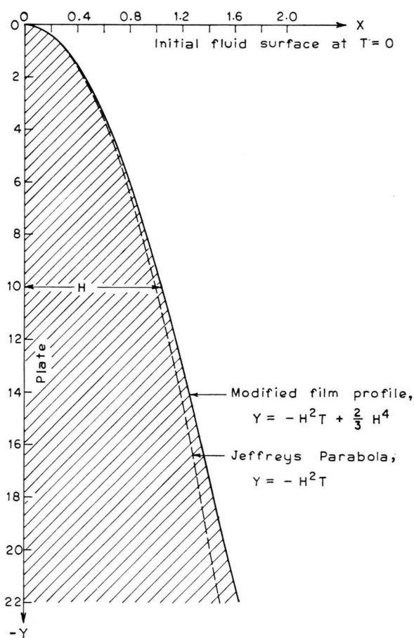
Fig. 1. Steady state film profiles at T=10 .
